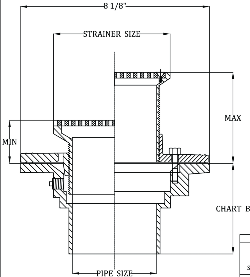
R-Round Strainer
