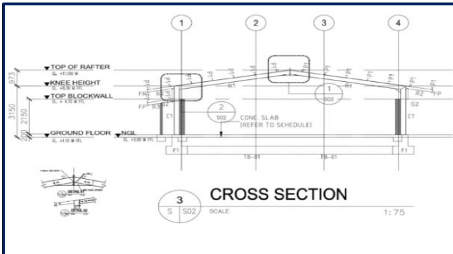
Steel Structures
