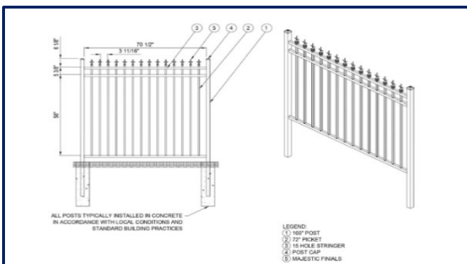
Steel Fencing
